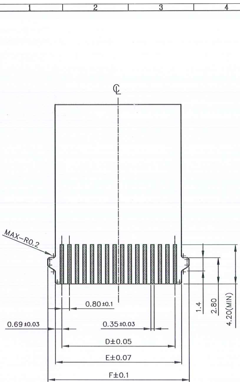
RECOMMENDED FFC DIMENSION
